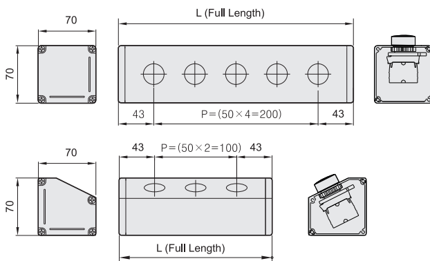
Dimensions (Unit : mm) Mounting hole layout \varnothing 22.5/25.5
